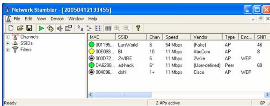
Figure 10-12: NetStumbler showing potentially unauthorized APs.
