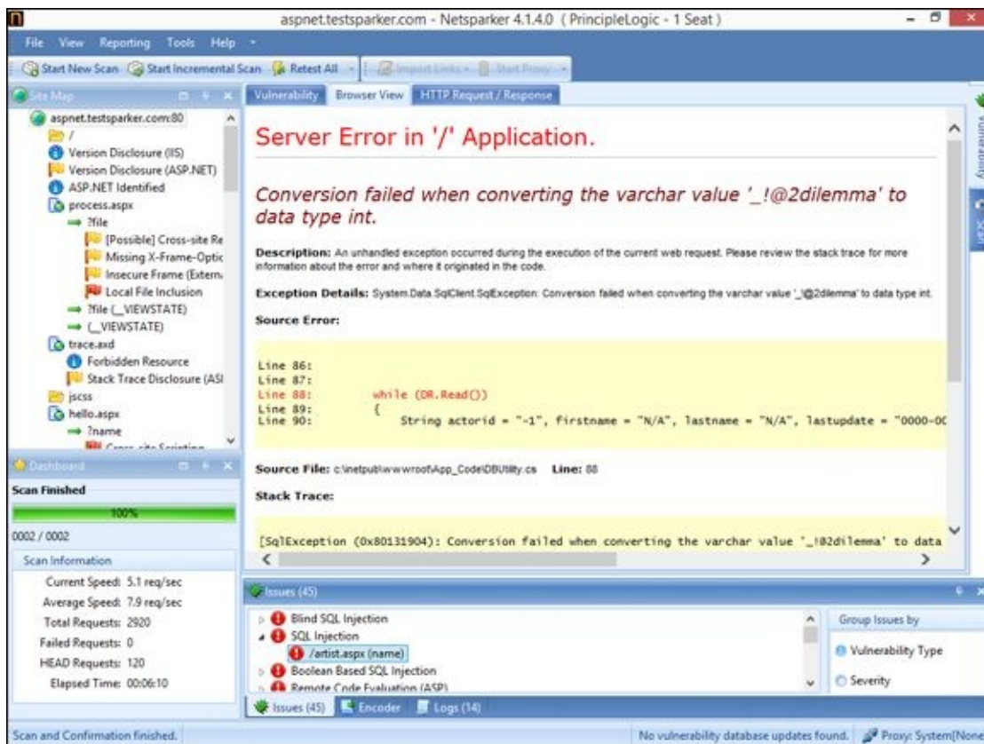
Figure 15-4: Netsparker discovered SQL injection vulnerabilities.
