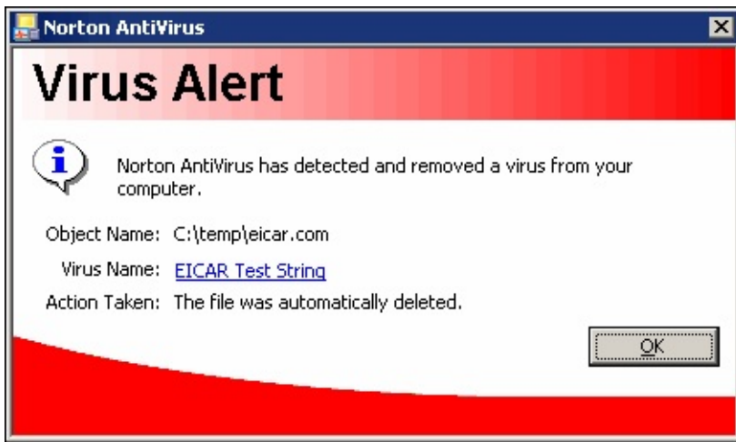
Figure 14-11: Using the EICAR test string to test antivirus software.
