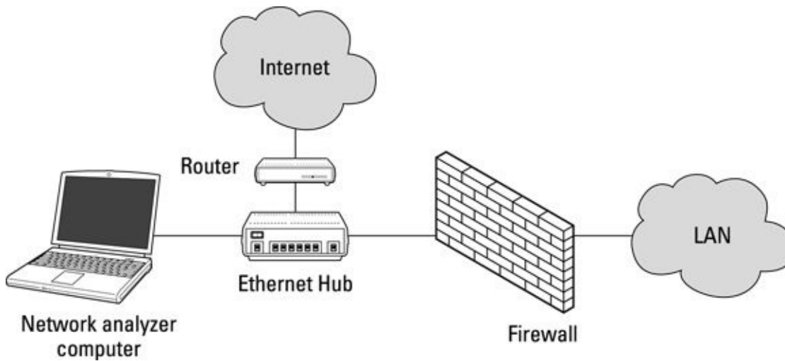
Figure 9-8: Connecting a network analyzer outside the firewall.
