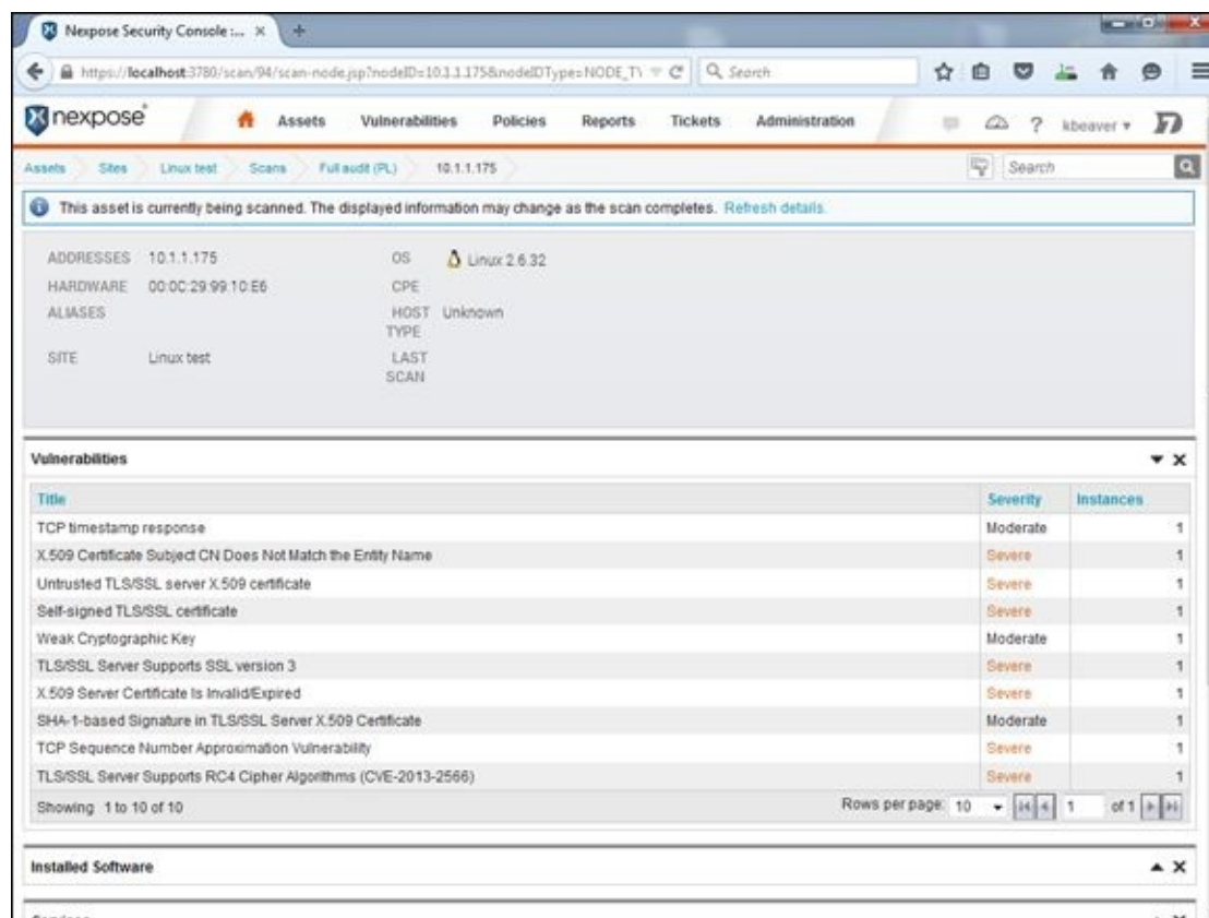
Figure 13-2: Using Nexpose to discover vulnerabilities with SSL.
