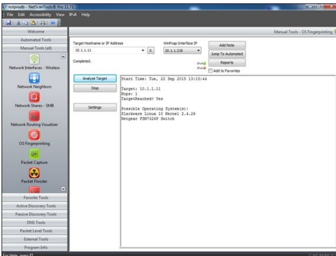
Figure 13-5: Using NetScan-Tools Pro to determine that Slackware Linux is likely running.
