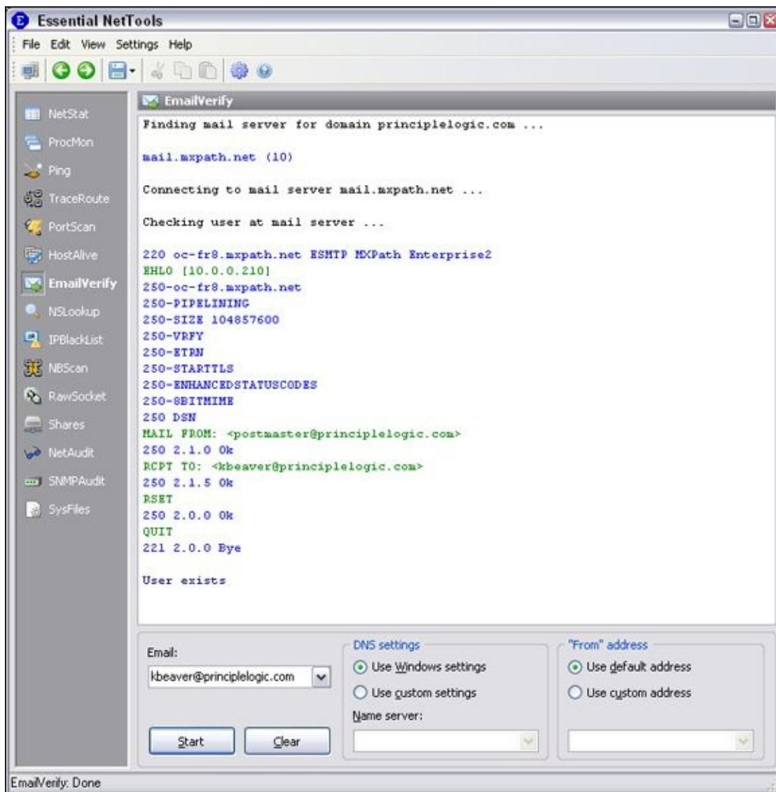
Figure 14-7: Using EmailVerify to verify an e-mail address.
