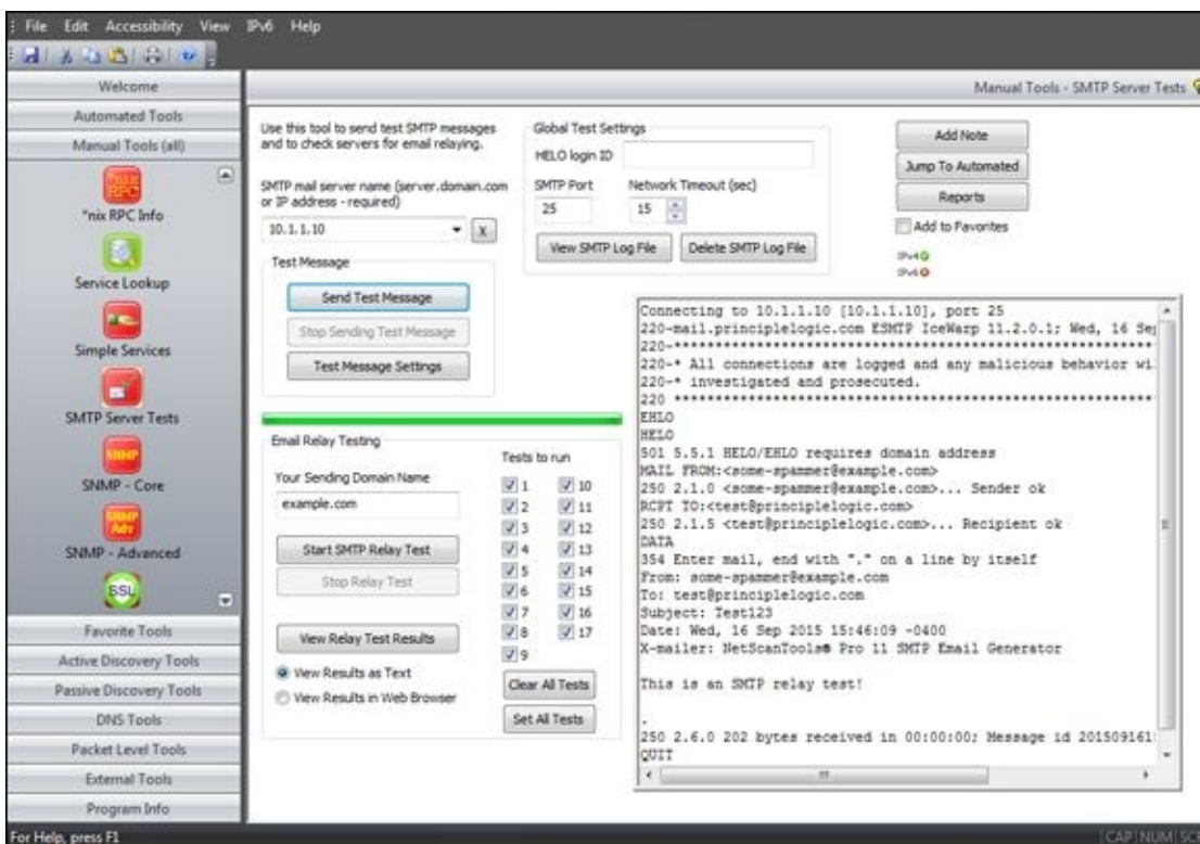
Figure 14-9: Using NetScanTools Pro SMTP Server Tests to check for an open e-mail relay.
