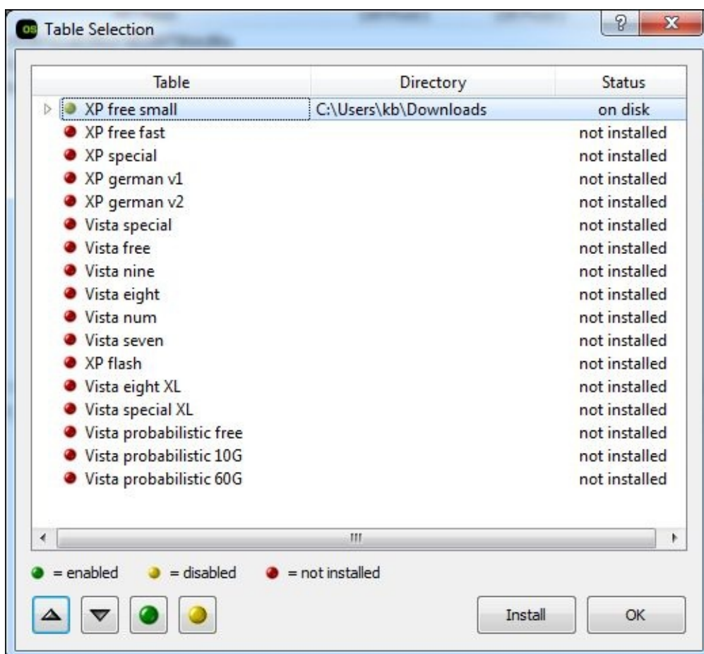
Figure 11-4: Loading the required hash tables in ophcrack.
