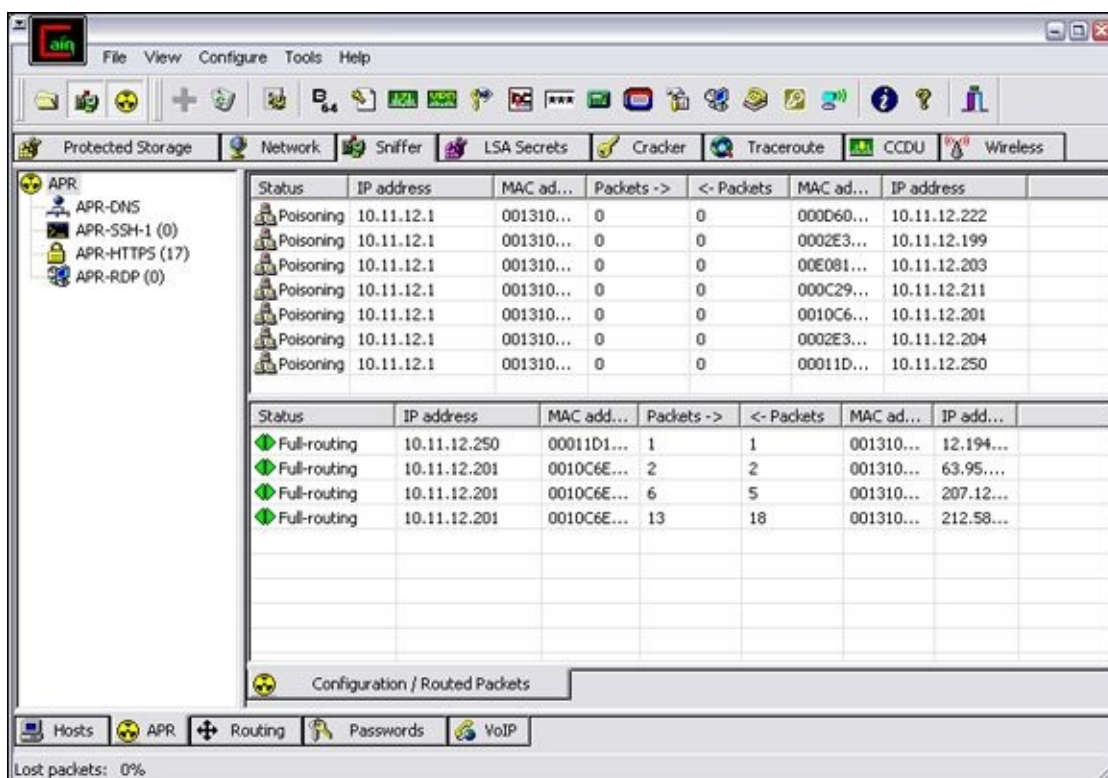
Figure 9-13: ARP poisoning results in Cain & Abel.
