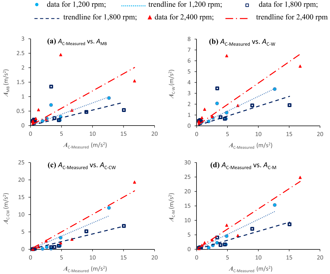
Fig. 8. The correlations in the frequency range of 20–125 Hz between the measured workpiece vibrations ( A_{C-Measured} ) for three different machine operating speeds and their corresponding vibrations estimated using T_W and T_C for R55 interface under a 30 N feed force: (a) A_{C-Measured} vs. machine body vibration ( A_{MB} ); (b) A_{C-Measured} vs. the estimated vibration transmitted from the machine to the workpiece ( A_{C-W} = \chi^* T_W^* A_{MB} , in which \chi = 3 ); (c) A_{C-Measured} vs. the vibration induced from the machine-transmitted vibration ( A_{C-CW} = T_C^* A_{C-W}^* \zeta/m_c , in which \zeta/m_c = 2.5 ); (d) A_{C-Measured} vs. the estimated workpiece vibration ( A_{C-M} = A_{C-W} + A_{C-CW} ).
