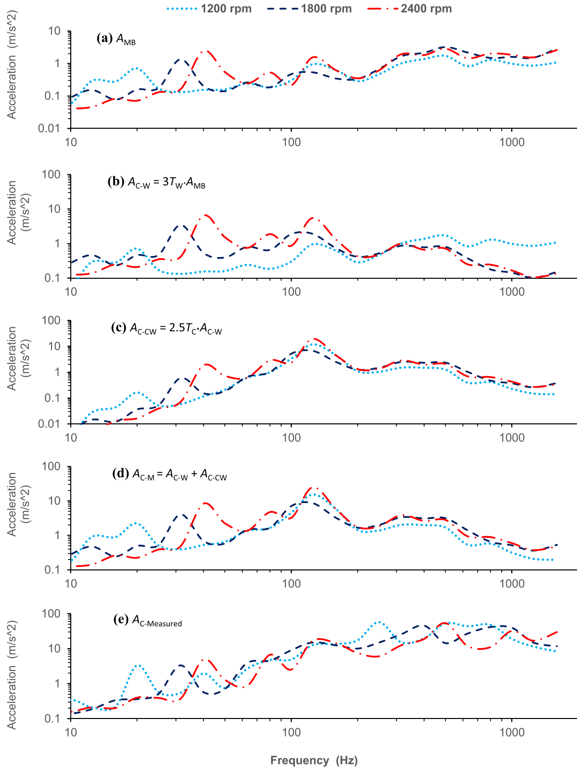
Fig. 7. Comparisons of the measured acceleration spectra at three different operation speeds with those estimated using T_W and T_C for R55 interface under 30 N feed force: (a) the measured machine body acceleration ( A_{MB} ) (Chen et al., 2017); (b) the estimated acceleration transmitted from the machine to the workpiece ( A_{C-W} = \chi \cdot T_W \cdot A_{MB} , in which \chi = 3 ); (c) the acceleration induced from the machine-transmitted vibration ( A_{C-CW} = T_C \cdot A_{C-W} \cdot \zeta / m_c , in which \zeta / m_c = 2.5 ); (d) the model-estimated workpiece acceleration ( A_{C-M} = A_{C-W} + A_{C-CW} ); (e). The measured workpiece acceleration ( A_{C-Measured} ) (Chen et al., 2017).
