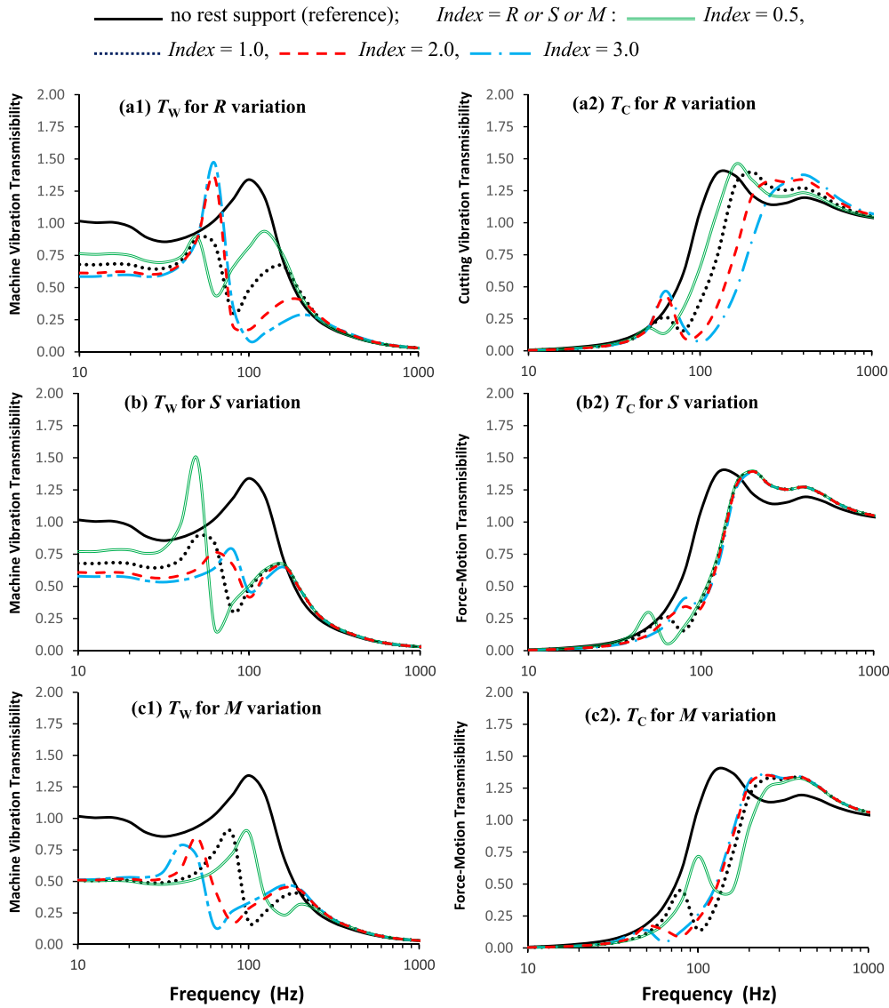
Fig. 15. The effects of an independent rest support on the workpiece responses predicted using the model shown in Fig. 3 (c) with X = 1 and Y = 1 in the machine body model: (a) the effects of rest contact properties ( K_R = R K_1 , C_R = R C_1 ) for given rest support mass ( m_R = 1.0 kg) and support properties ( K_S = K_1 , C_S = C_1 ); (b) the effects of rest support properties ( K_S = S K_1 , C_S = S C_1 ) for given rest support mass ( m_R = 1.0 kg) and rest contact properties ( K_R = K_1 , C_R = C_1 ); (c) the effects of rest support mass ( m_R = M kg) for given rest contact and support properties ( K_R = 2K_1 , C_R = 2C_1 , K_S = 2K_1 , C_S = 2C_1 ).
