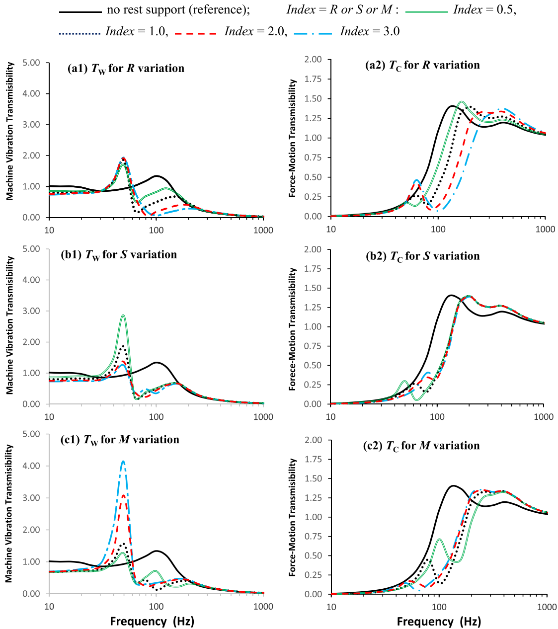
Fig. 13. The effects of a rest support on workpiece responses predicted using the model shown in Fig. 3(b) with X = 1 and Y = 1 in the machine body model: (a) the effects of rest contact properties ( K_R = RK_1 , C_R = RC_1 ) for given rest mass and support properties ( M = 1 , S = 1 ); (b) the effects of rest support properties ( K_S = SK_1 , C_S = SC_1 ) for given rest mass and contact properties ( M = 1 , R = 1 ); (c) the effects of rest mass ( m_R = M kg) for given rest contact and support properties ( R = 2 , S = 2 ).
