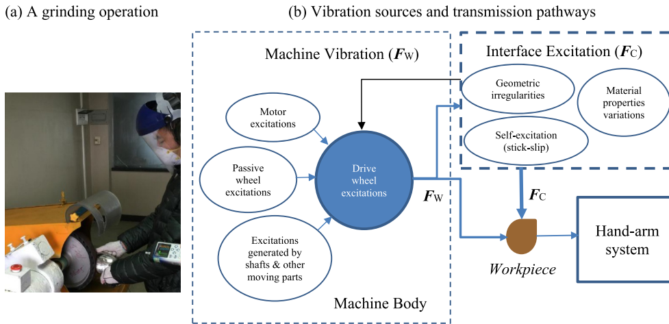
Fig. 1. The simulation of a grinding operation on a belt grinding machine: (a) a pictorial view of the grinding of a workpiece held by two hands of a worker (Chen et al., 2017); (b) vibration sources and transmission flow-chart, in which F_W represents the overall equivalent machine vibration force acting on the grinding drive wheel of the machine, and F_C represents the overall equivalent cutting vibration force acting on the workpiece; and (c) a model of the grinding machine-workpiece-hand-arm system (Dong et al., 2018), in which z represents the displacement of each lumped mass in the system, K represents connecting stiffness in the system, and C represents its damping values.
