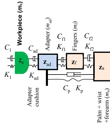
Fig. 2. A portion of the system model with added adapters: (a) the adapter ( m_{ad} ) with a vibration absorber ( m_{ab} , K_{ab} , C_{ab} ) held by the hands; (b) suspended adapter ( m_{ad} ) held by the hands and with some cushioning ( K_{ad} , C_{ad} ) between the workpiece and the adapter.
